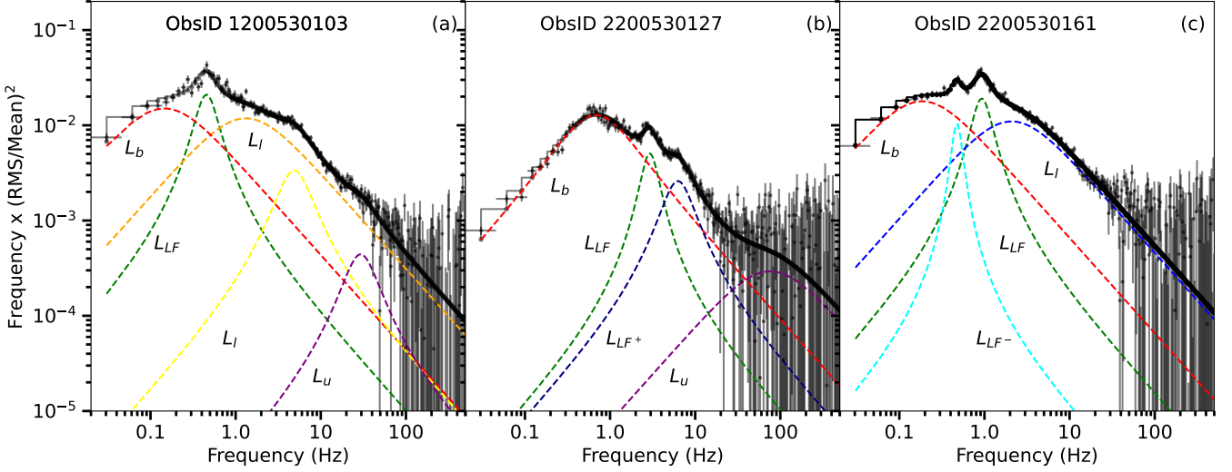
Figure 3. Three representative power spectra of observations with type-C QPOs of the outburst of MAXI J1348–630 during the rise (panel (a)), decay (panel (b)) and first reflare of the outburst (panel (c)). Dashed lines represent the best fit Lorentzians. The different components are identified with a name based on previous works on time variability in low-mass X-ray binaries.
