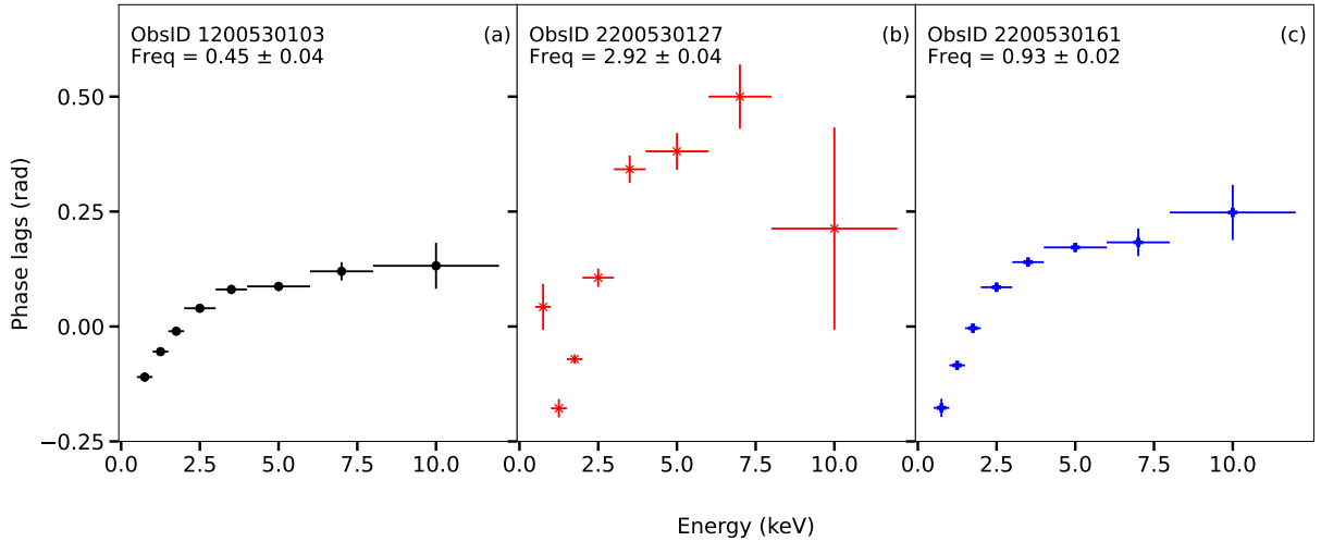
Figure 11. Representative examples of the lag spectra of the type-C QPO in MAXI J1348–630. Colours and symbols are the same as in Fig. 1.
