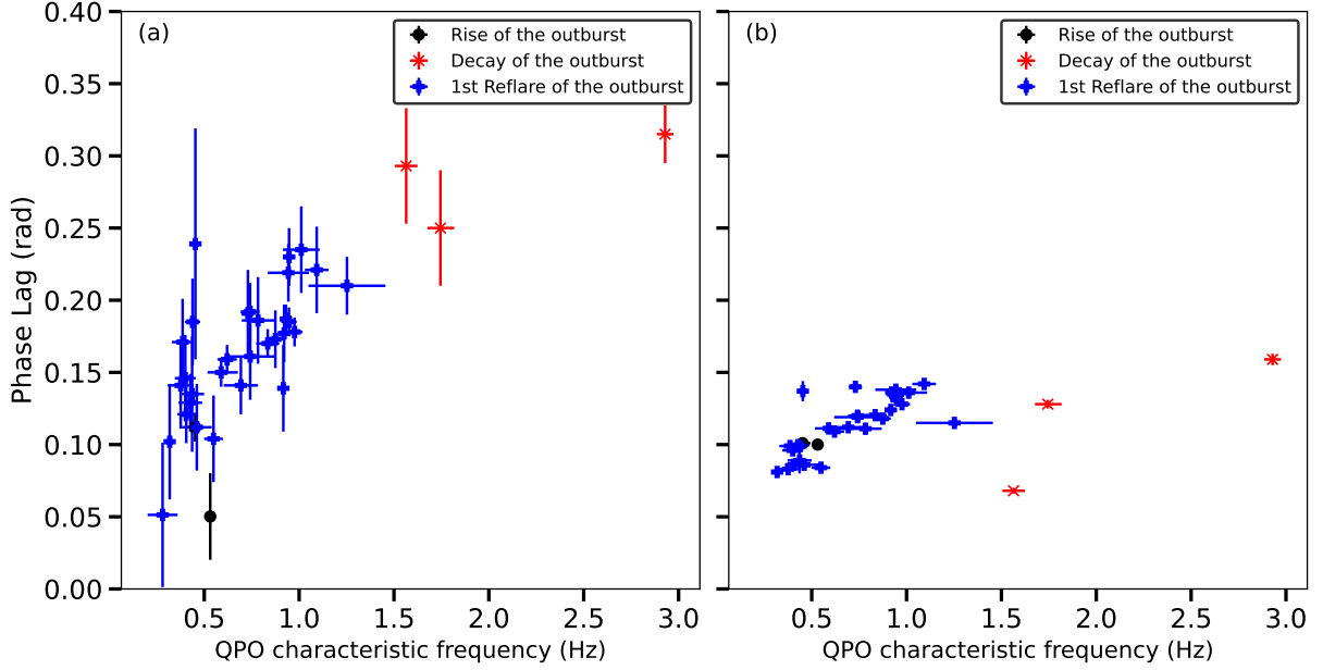
Figure 10. Phase lags as a function of the QPO frequency for the type-C QPO in MAXI J1348–630. (a): Lags obtained with the new method described in Section 2. (b): Average lags computed within the FWHM around the QPO characteristic frequency. Colours and symbols are the same as in Fig. 1.
