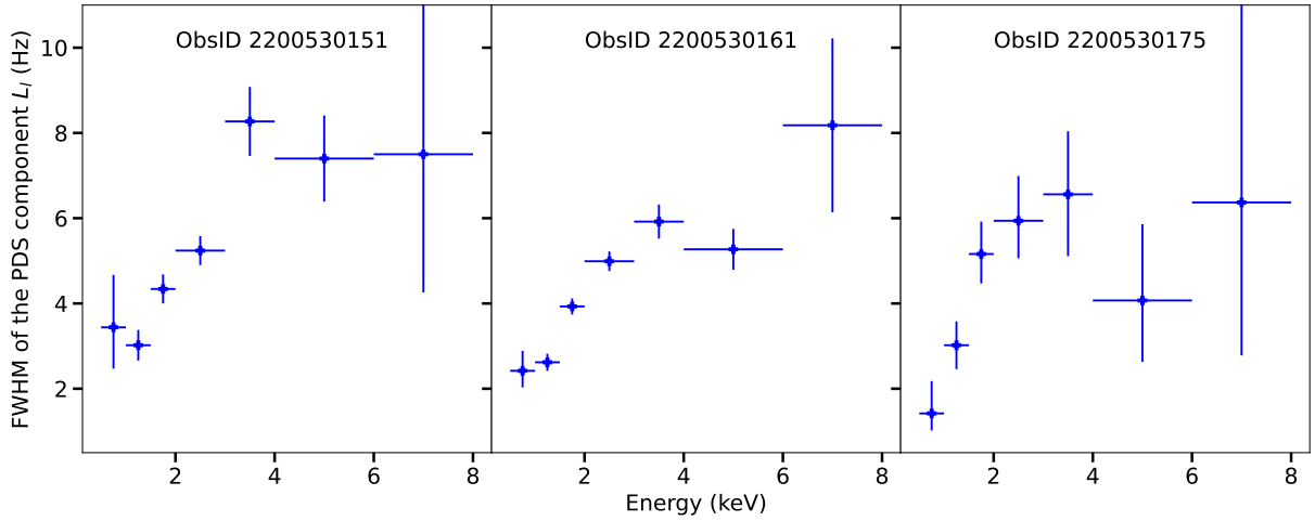
Figure 8. Energy dependence of the high-frequency broad component L_I of the PDS of the reflare.
