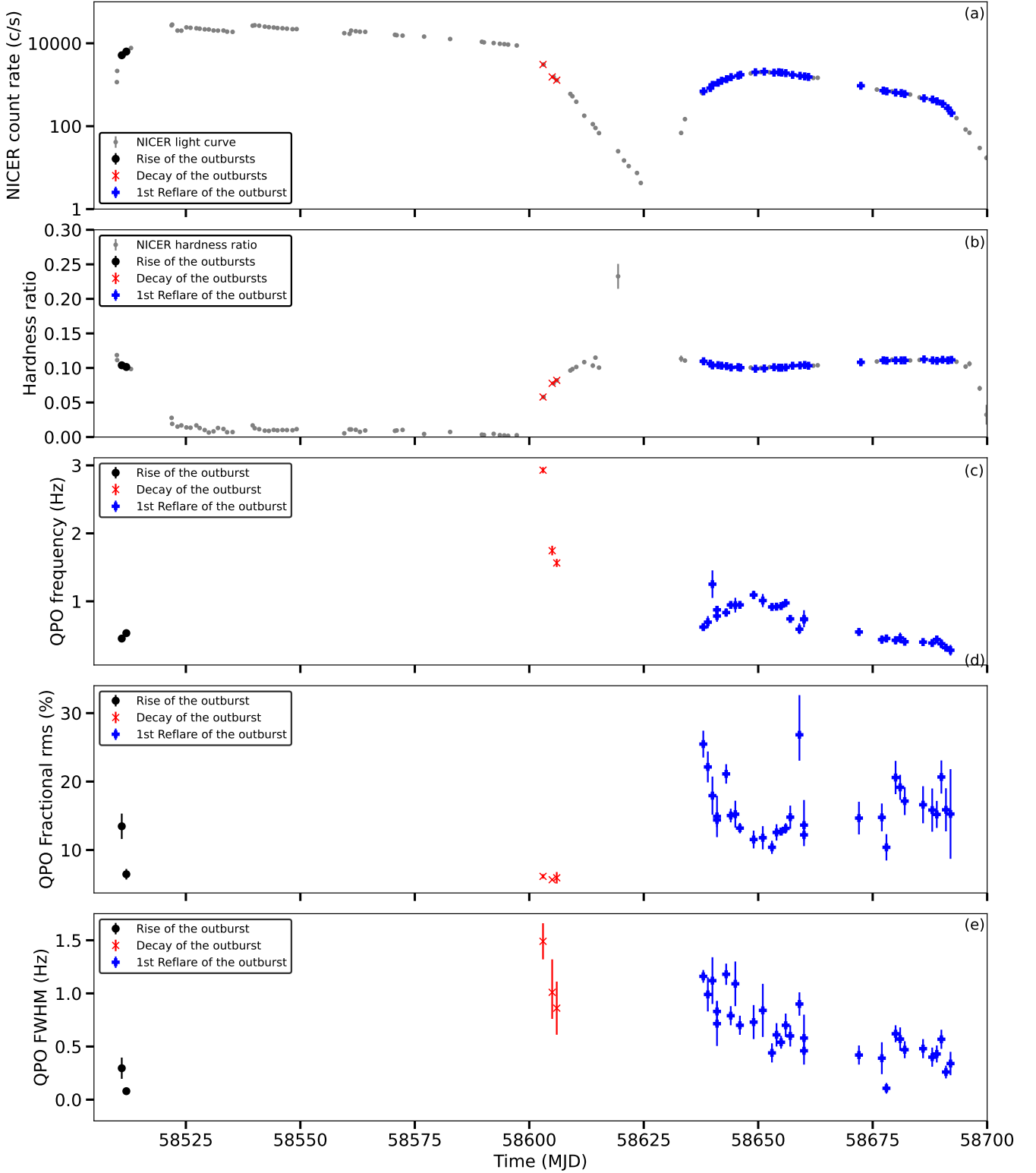
Figure 1. Panel (a): NICER light curve of MAXI J1348–630. Panel (b): Temporal evolution of the hardness ratio of MAXI J1348–630. Panel (c): Temporal evolution of the QPO frequency. Panel (d): Temporal evolution of the fractional rms amplitude of the QPO. Panel (e): Temporal evolution of the FWHM of the QPO. Black, red and blue symbols represent the data corresponding to the rise, the decay and the first reflare of the outburst, respectively. Grey symbols represent the full NICER light curve (panel (a)) and the full temporal evolution of the hardness ratio (panel (b)).
