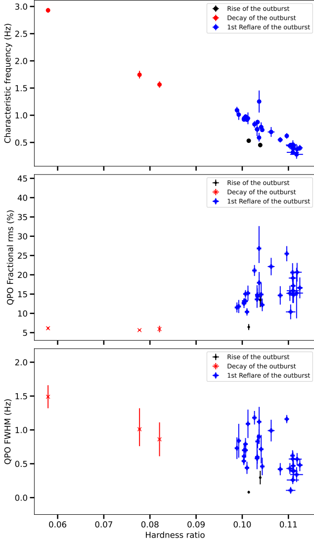
Figure 6. Frequency (top panel), fractional rms amplitude (middle panel) and FWHM (bottom panel) of the type-C QPO vs. the hardness ratio.
