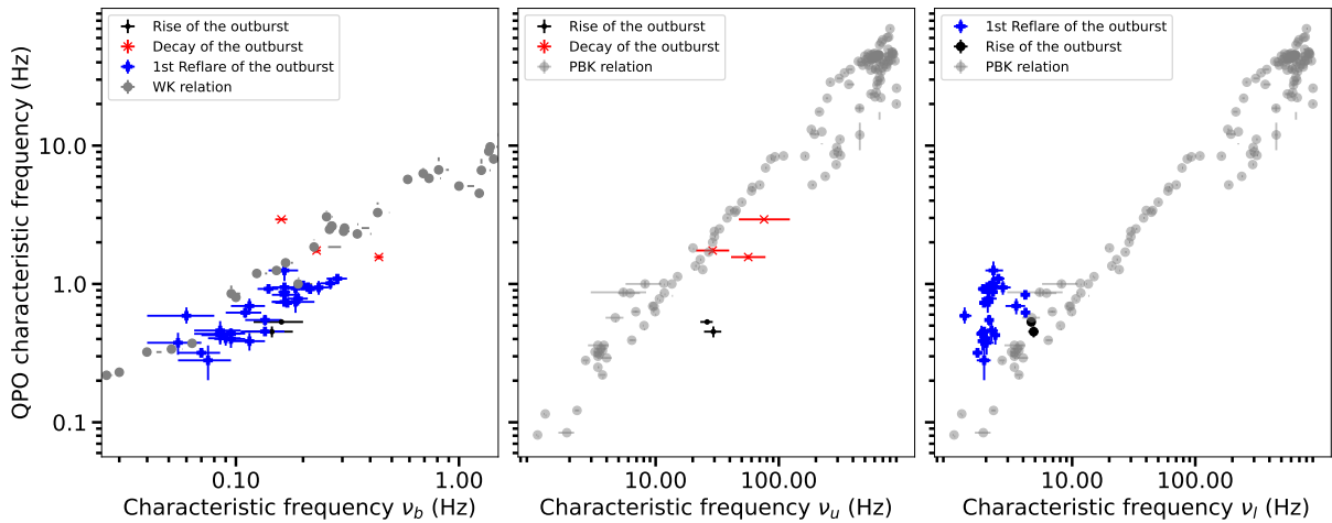
Figure 5. Relation of the frequencies of L_{LF} with L_b (left panel); L_u (middle panel) and L_l (right panel). Black, red and blue symbols are the same as in Fig. 1. Grey symbols represent the PBK relation with data from Psaltis et al. (1999), Nowak (2000), Homan et al. (2001), Belloni et al. (2002b) and Nowak et al. (2002) in the middle panel. Grey symbols represent the WK relation as shown in Wijnands & van der Klis (1999) in the left and right panels.
