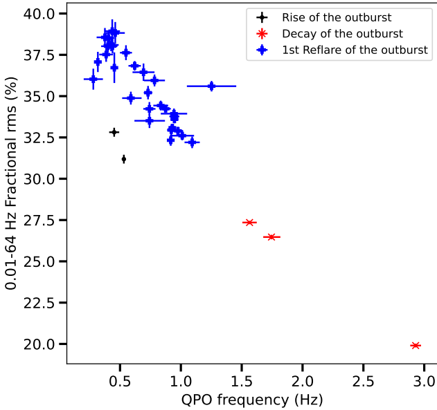
Figure 4. Fractional rms amplitude in the 0.01–64 Hz frequency range vs QPO frequency. Colours and symbols are the same as in Fig. 1.
