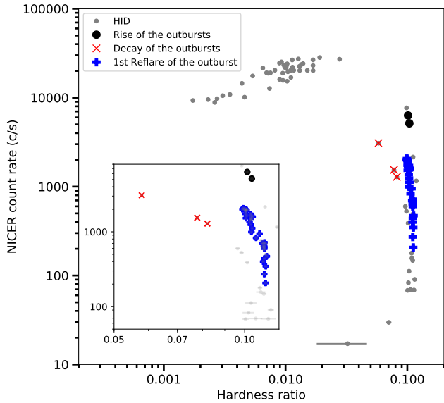
Figure 2. HID of MAXI J1348–630. Grey: Data points for the full outburst and reflares. Colours and symbols are the same as in Fig. 1.
