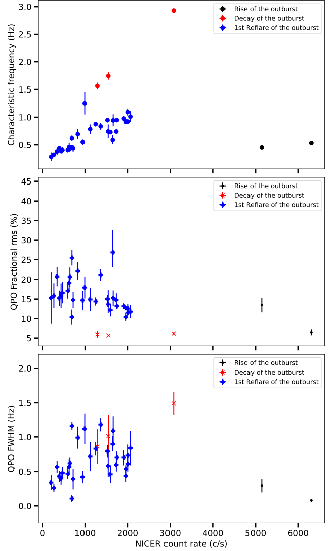
Figure 7. Frequency (top panel), fractional rms amplitude (middle panel) and FWHM (bottom panel) of the type-C QPO vs. the count rate.
