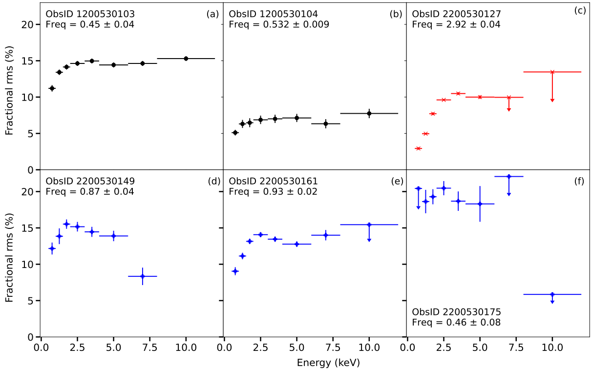
Figure 9. Representative examples of the rms spectra of the type-C QPO in MAXI J1348–630. Colours and symbols are the same as in Fig. 1. Arrows represent the 95% confidence upper limits of the fractional rms amplitude. On panel (d), there is an upper limit of 82% at 10 keV that is not shown due to the selected range for the fractional rms in the y-axis.
