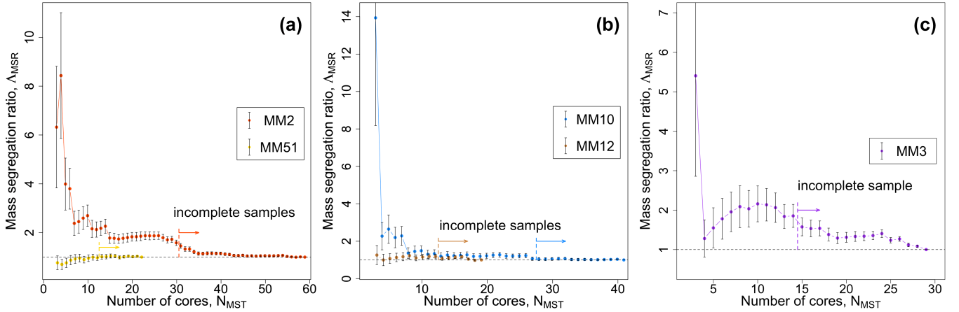
Fig. 8. Mass segregation ratio of cores in the W43-MM2&MM3 subregions. Computed from Eq. (7), they are measured in the MM2 and MM51 subregions ( panel a ), in MM10 and MM12 ( panel b ), and in the MM3 subregion ( panel c ). Error bars are the \pm 1\sigma uncertainties. Right arrows and vertical dashed lines locate the 90% completeness levels of the subregion catalogs of cores (see Table 2). Values well above \Delta_{\text{MSR}} \approx 1 (black dashed horizontal line) robustly suggest mass segregation in MM2, MM3, and MM10 (see Table 3).
