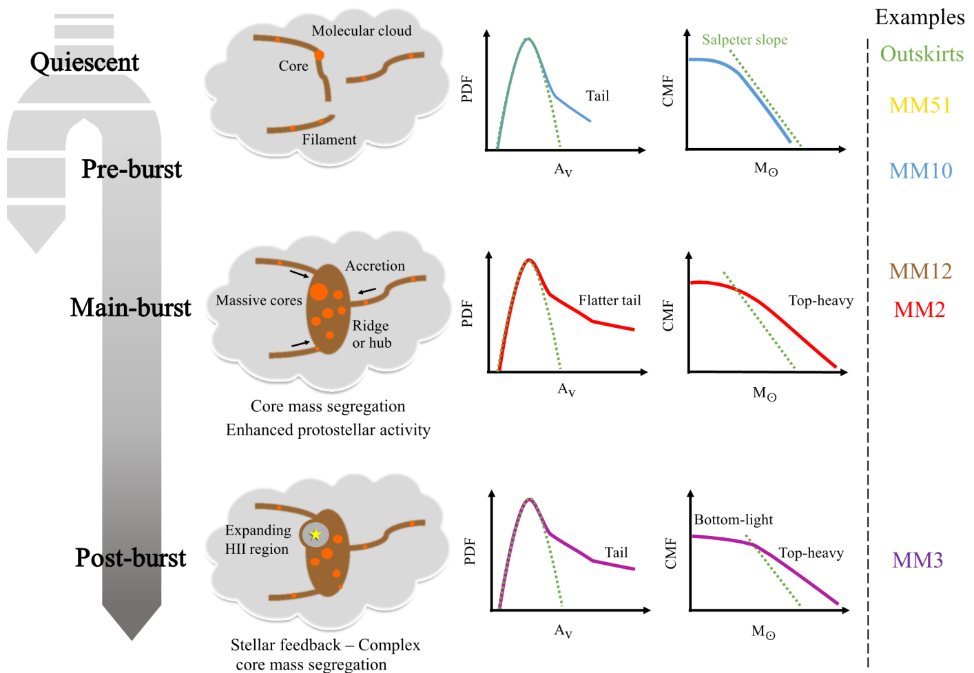
Fig. 11. Schematic evolutionary diagram of subregions in dynamical star-forming clouds, which are qualified as either quiescent or by following the different phases before, during, and after their main star formation event: pre-burst, main burst and post-burst. Their characteristics, including cloud column density \eta -PDF, CMF, and core mass segregation are illustrated. Top panels: Subregions in quiescent or pre-burst regimes present a \eta -PDF tail close to that found in low-mass star-forming regions and a CMF high-mass end close to the Salpeter slope. Central panels: Subregions in their main burst regime harbor an enhanced star-formation activity and strong core mass segregation. They display an \eta -PDF with a much flatter second tail as well as a top-heavy CMF. Bottom panels: Post-burst subregions, under the influence of stellar feedback, have less sustained star formation activity and more complex core mass segregation. They also present an \eta -PDF with a flat second tail, and a CMF which is both top-heavy and bottom-light. The location on the time sequence of the W43-MM2&MM3 subregions are given to summarize the result of present article.
