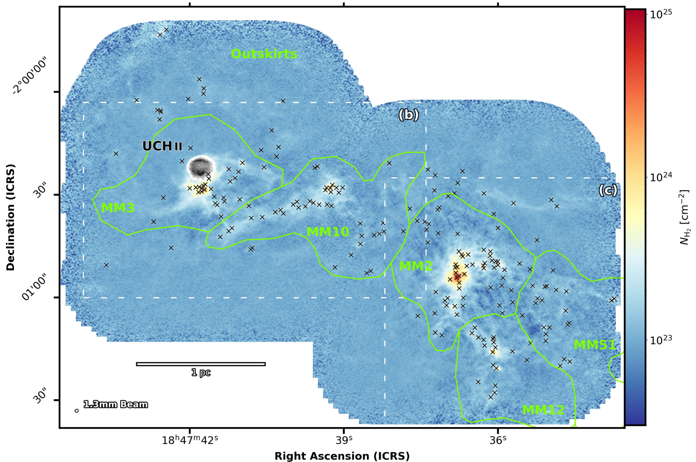
Fig. 1. The W43-MM2&MM3 mini-starburst ridge traced by its column density (color scale), derived from the ALMA 1.3 mm continuum image of Pouteau et al. (2022). It hosts a rich cluster of 205 cores (gray crosses) reported by Pouteau et al. (2022) and the ultra-compact H II (UCH II) region of W43-MM3, traced by its H41 \alpha emission line (Galván-Madrid et al. in prep., gray scale) and where the column density is not computed. Green polygons outline the W43-MM2&MM3 subregions defined in Sect. 2.2. The ellipse in the lower left corner indicates the 0.46'' angular resolution of the column density image while the scale bar indicates the length scale at a distance of 5.5 kpc. a) White dashed boxes outline the zooms-ins of b – c .
