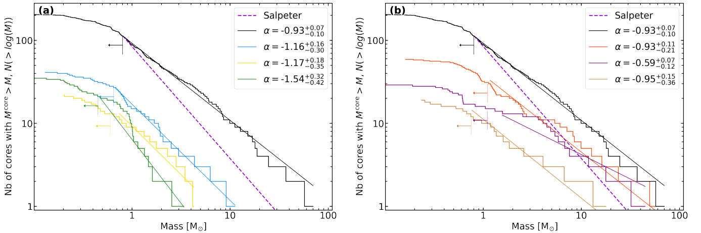
Fig. 4. CMFs of the W43-MM2&MM3 subregions, plotted in their cumulative form, with shapes at high-mass end varying from steeper or close to the Salpeter slope of the canonical IMF (MM10, MM51, and Outskirts, panel a ) to top-heavy (MM2, MM3, and MM12, panel b ). CMFs (colored histograms) are fitted by single power-laws of the form N(> \log(M)) \propto M^{\alpha} (lines), above the associated 90% completeness limits (left arrows and vertical lines, see Table 2) and using a bootstrapping method which uses a MLE method (see Sect. 3.1.2). The high-mass end of the canonical IMF, which has a power-law index of \alpha_{\text{IMF}} = -1.35 (dashed magenta lines, Salpeter 1955) is shown for comparison. The top-heavy CMF of the W43-MM2&MM3 ridge (black histogram) mostly originates from that of the MM2 subregion. The MM3 CMF is complex, being both top-heavy and bottom-light.
