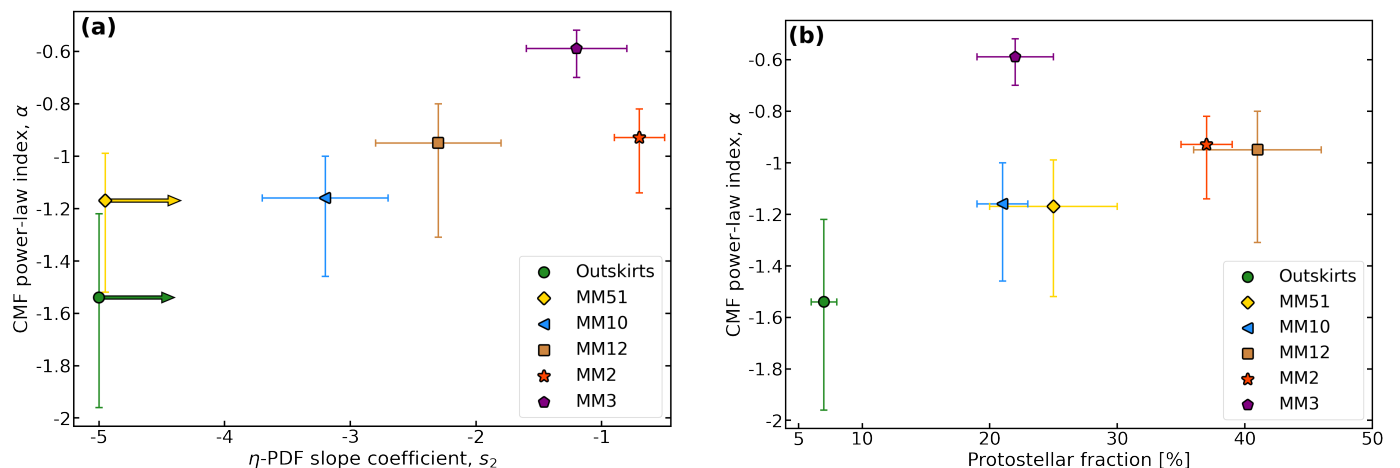
Fig. 9. For each W43-MM2&MM3 subregion, the power-law index of the CMF high-mass end is plotted against the slope coefficient of the second \eta -PDF tail ( panel a ) and the protostellar fraction ( panel b ). Horizontal arrows represent lower limits for s_2 in panel a . We avoid fitting the correlation trends observed in panels a–b because they rely on a too few subregions.
