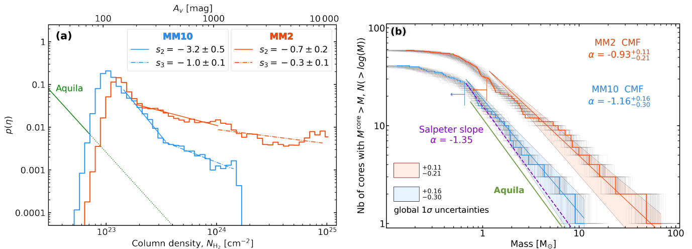
Fig. 10. Two prototypical subregions of W43-MM2&MM3, MM2 (red pencil) and MM10 (blue pencil), compared with Aquila (green pencil). Panel (a): \eta -PDF histograms, whose tails (colored segments) are fitted with power-laws. Green solid and dotted lines correspond to the observed and extrapolated column density ranges from Könyves et al. (2015). While the \eta -PDF of the MM2 subregion displays a flat power-law tail, those of MM10 and Aquila are much steeper. Panel (b): Cumulative CMF histograms, whose high-mass ends are represented by power-laws (colored segments) and their 1\sigma global uncertainties (colored areas, see definition in Sect. 3.1.2). While the MM2 subregion exhibits a top-heavy CMF, MM10 and Aquila have steeper CMF high-mass ends, with power-law indices close to the Salpeter slope (dashed magenta line).
