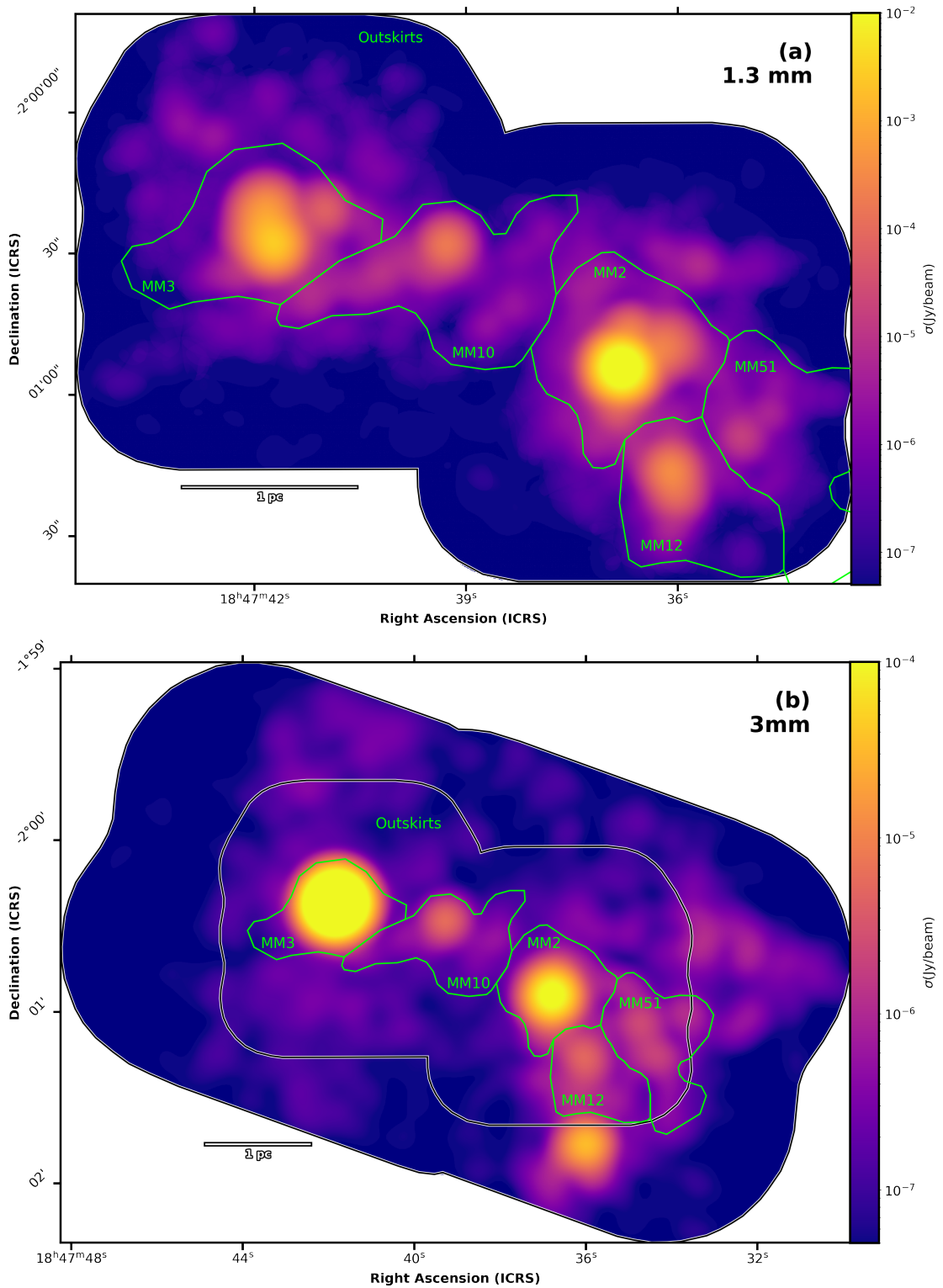
Fig. 2. Subregions of 0.5 – 1 pc sizes identified in the W43-MM2&MM3 ridge from the ALMA 12 m array denoised bsens continuum images of Pouteau et al. (2022) at 1.3 mm (panel a) and 3 mm (panel b). A multi-scale decomposition was performed, decomposition scales of \sim 4\text{--}7'' were chosen and subregion outlines (green contours) were set to follow inflection points in the column density distribution. Subregions are labelled MM2, MM3, MM10, MM12 and MM51 following the names of fragments extracted from \sim 10'' resolution (sub)millimeter images (Motte et al. 2003). The remaining subregion at 1.3 mm is labelled Outskirts. The white contour outlines the 1.3 mm coverage in panel (b) and a 1-pc scale bar is shown in the lower-left corner of each image.
