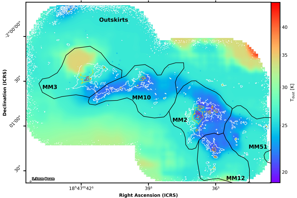
Fig. A.1. Dust temperature image of the W43-MM2&MM3 protocluster cloud, taken from Pouteau et al. (2022). It combines a 2.5'' resolution dust temperature image computed from a bayesian SED fit for fluxes ranging from 70 \mu\text{m} to 3 mm (see Dell'Ova et al. in prep.) with the central heating and self-shielding of protostellar and pre-stellar cores, respectively, at 0.46'' resolution (see Sect. 4.2 of Pouteau et al. 2022, for more details). White, orange and red contours correspond to N_{\text{H}_2} levels defined in Fig. 1b–c. Black polygons indicate the subregions defined in Section 2.2 and the ellipse in the bottom left corner corresponds to the 1.3 mm beam.
