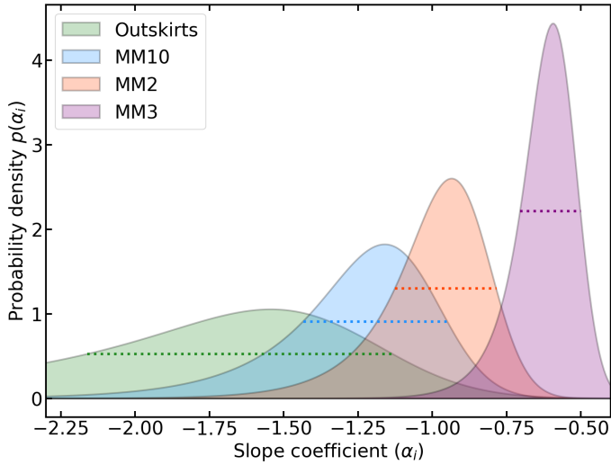
Fig. A.3. Bootstrapping probability density functions of the power-law indices measured for the CMF high-mass end of the MM2, MM3, MM10, and Outskirts subregions. Each distribution is fitted by an exponentially modified Gaussian with negative skewness. According to their 1\sigma width (dotted segments), subregions appear distinct except for MM10, whose highest probability part of the bootstrapping distribution overlap with both the MM2 and Outskirts subregions.
