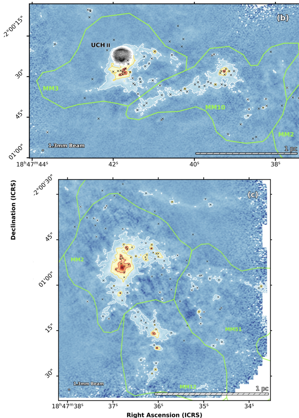
Fig. 1. (Continued) Zooms on the MM3 and MM10 subregions (b) and the MM2, MM12 and MM51 subregions (c). White, orange, and red contours correspond to column densities of 1.5 , 3.5 , and 10 \times 10^{23} \text{ cm}^{-2} . Pixels located between the white and orange, and white and red, contours constitute the s_2 tails of the MM10 and MM51, and the MM2, MM3, and MM12 subregions, respectively.
