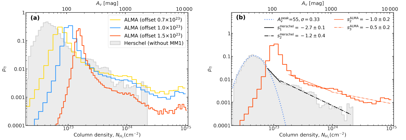
Fig. A.2. Comparison of the \eta -PDFs produced from the column density images of Herschel /HOBYS covering W43-Main (18.1''-beam, without W43-MM1, shaded-gray histogram) and of ALMA-IMF toward W43-MM2&MM3 (0.51'' \times 0.40''-beam, colored histograms). Panel (a) : Determination of the background column density of W43-MM2&MM3 that best reconciles the ALMA and Herschel \eta -PDFs: 1 \times 10^{23} \text{ cm}^{-2} . \eta -PDFs are built with this column density offset (blue histogram) and the lower and upper limits of the offset uncertainty (yellow and red histograms, respectively). The Herschel \eta -PDF has been multiplied by 4 to emphasize its relative agreement with the ALMA \eta -PDF. Panel (b) : \eta -PDF tails of Herschel /HOBYS and ALMA-IMF with consistent power-law indices: s_2^{\text{Herschel}} = -1.2 \pm 0.4 (dotted black segment) and s_2^{\text{ALMA}} = -1.0 \pm 0.2 (continuous red segment). The first \eta -PDF tail with power-law index s_1 (continuous black segment) is only traced by the Herschel image, the third tail with power-law index s_3 (dotted red segment) is mainly traced by ALMA.
